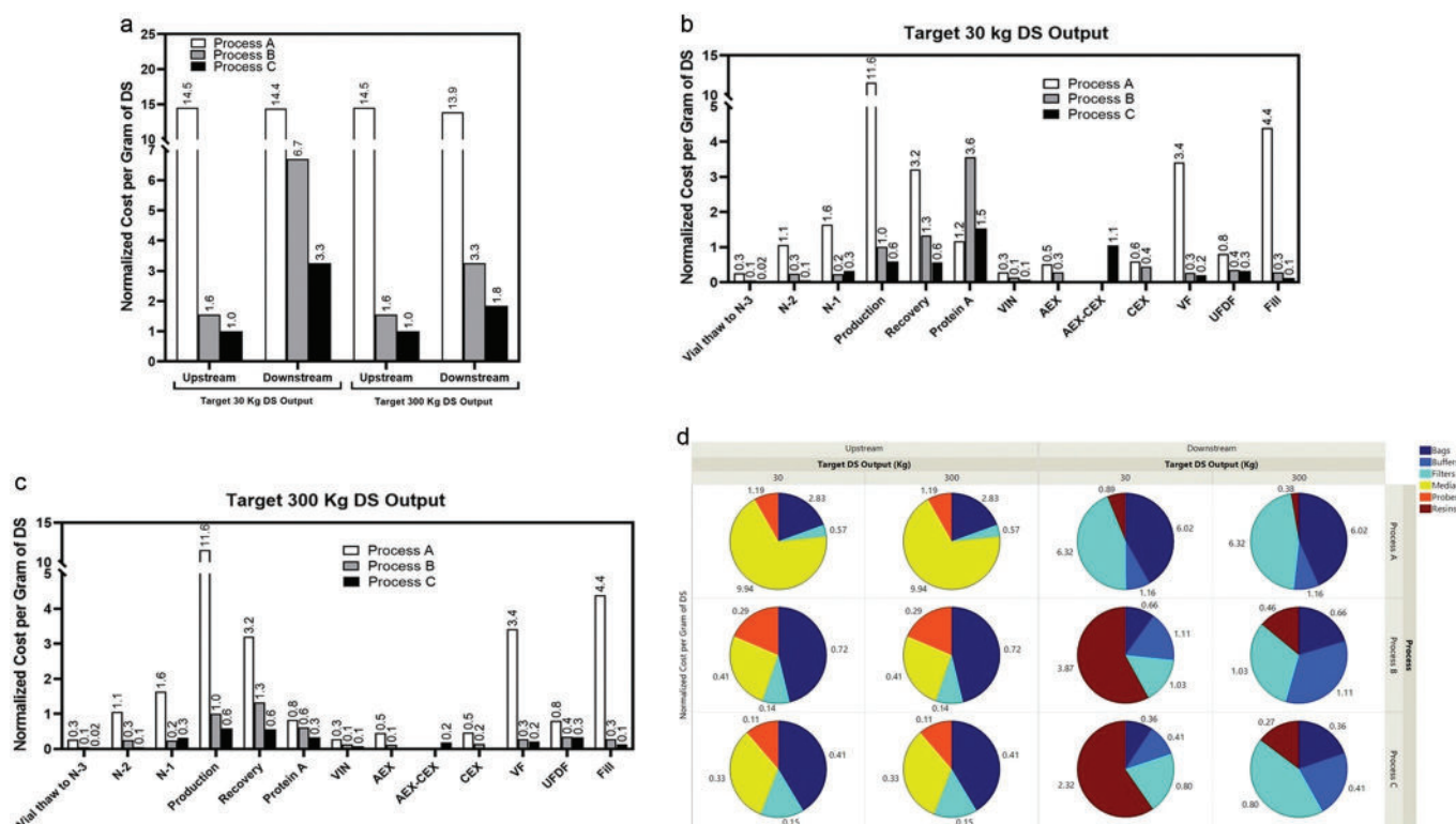
Figure 7. Consumables (resins, filters, bags, media, buffers, and probes) costs for Process A, Process B, and Process C assumed to be all at 2000-L bioreactor scale: (a) upstream and downstream; step costs for (b) 30 kg and (c) 300 kg DS output, respectively; (d) breakdown cost.
