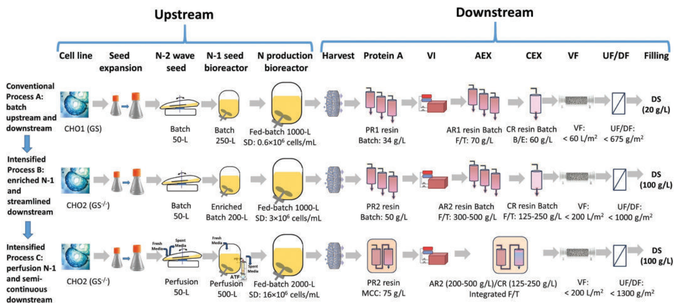
Figure 1. Biomanufacturing diagrams for Process A (conventional fed-batch at 1000-L scale, n = 5 ), Process B (intensified fed-batch by enriched N-1 at 1000-L scale, n = 8 ), and Process C (intensified fed-batch by perfusion N-1 at 2000-L scale, n = 3 ).
